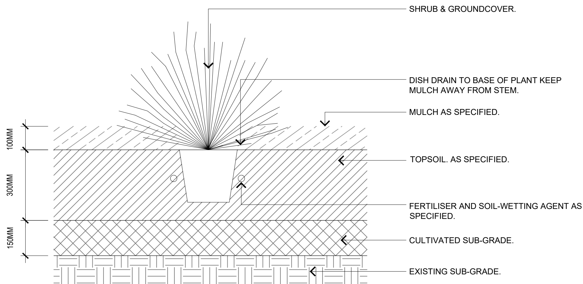
LD02 TYPICAL PLANTING DETAIL 1:10@A1
