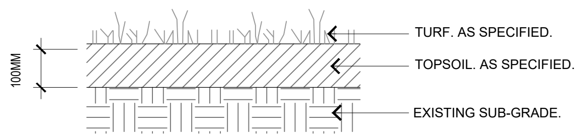
LD01 TYPICAL TURF DETAIL 1:10@A1
