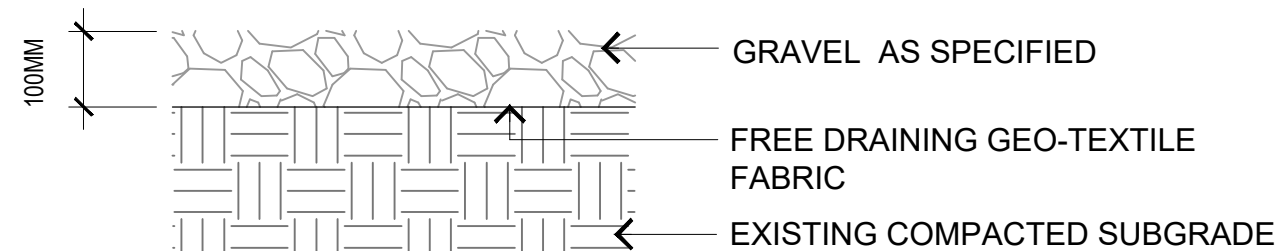
LD04 TYPICAL GRAVEL MULCH DETAIL 1:10@A1
