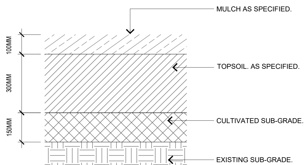
LD03 TYPICAL MULCH DETAIL 1:10@A1
