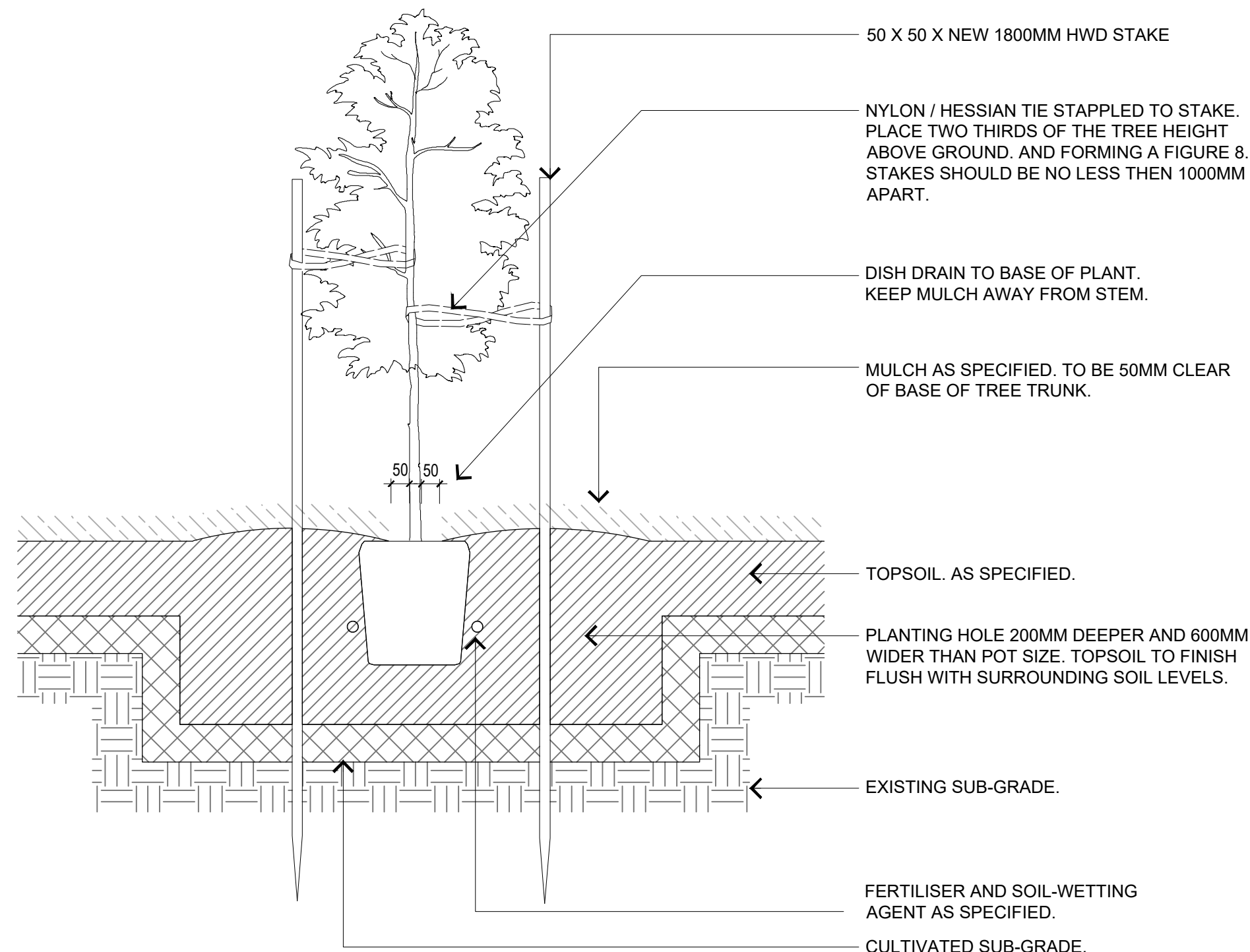
LD04 TYPICAL DETAIL: TREE PLANTING IN MULCH 1:20 @ A1
